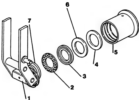
Fig. 44 Sleeve, guide lever assembly and bearing assembly
